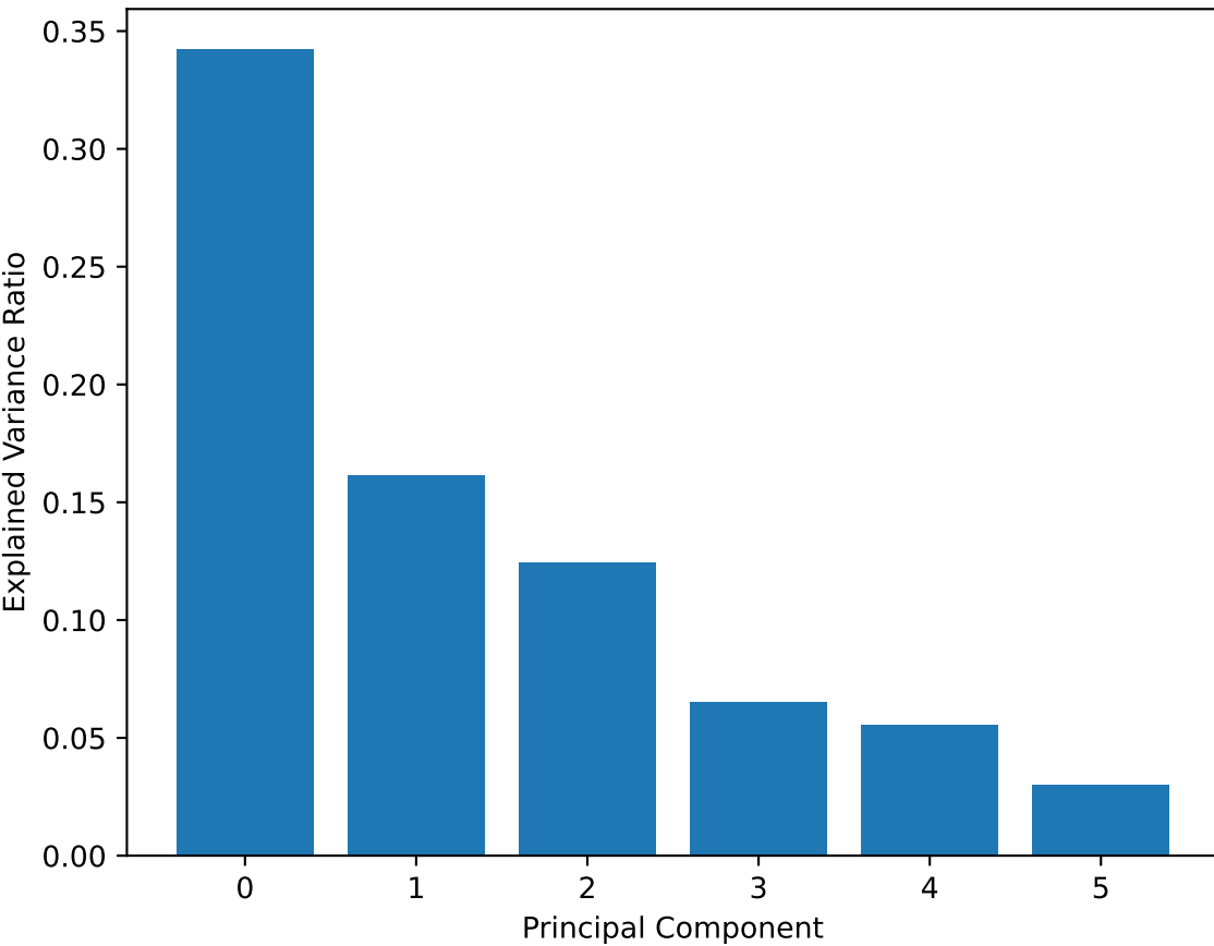
Individual Explained Variance
