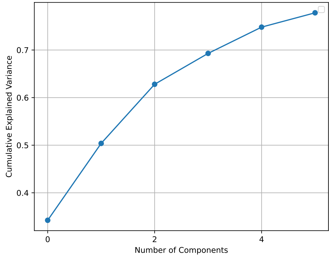
Cumulative Explained Variance
